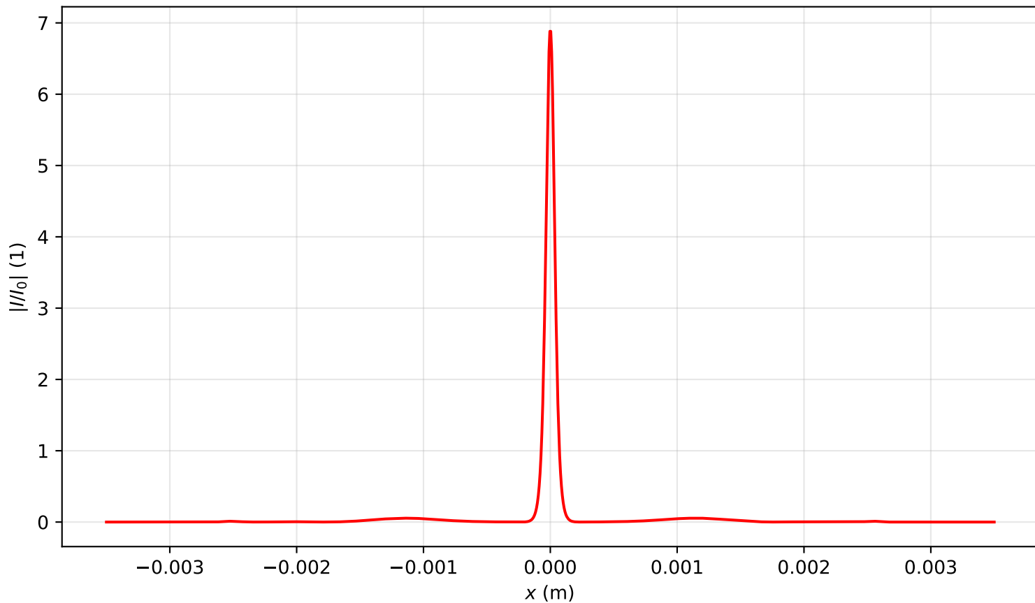
Intensity profile I(x, y = 0, z = 0.955)/I_0 , P_{in}=8.0P_{cr} , artificial time
